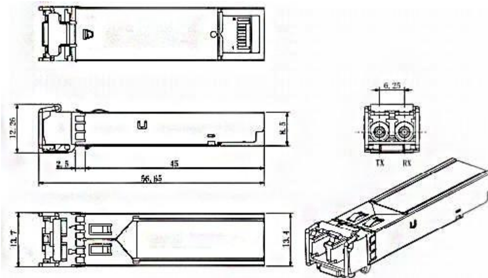
Figure 6. Mechanical Drawing
